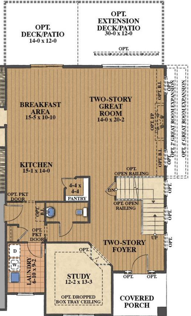
INCLUDED FIRST FLOOR LAYOUT
