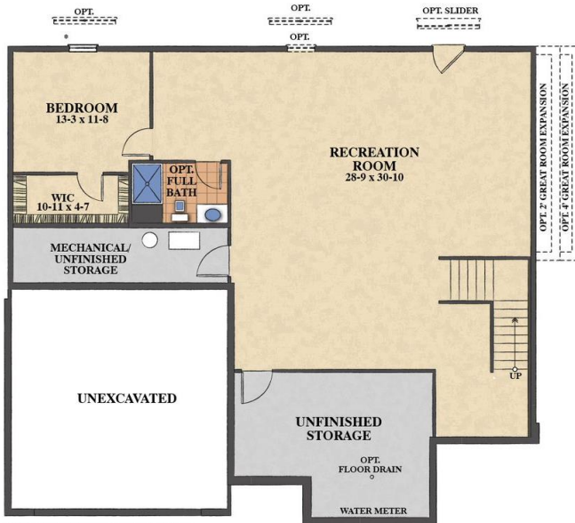
OPTIONAL FINISHED BASEMENT LAYOUT
