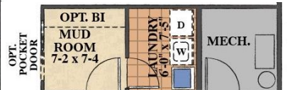
OPT. PREMIUM MUD ROOM LAYOUT (W/ SLAB PLAN ONLY)
