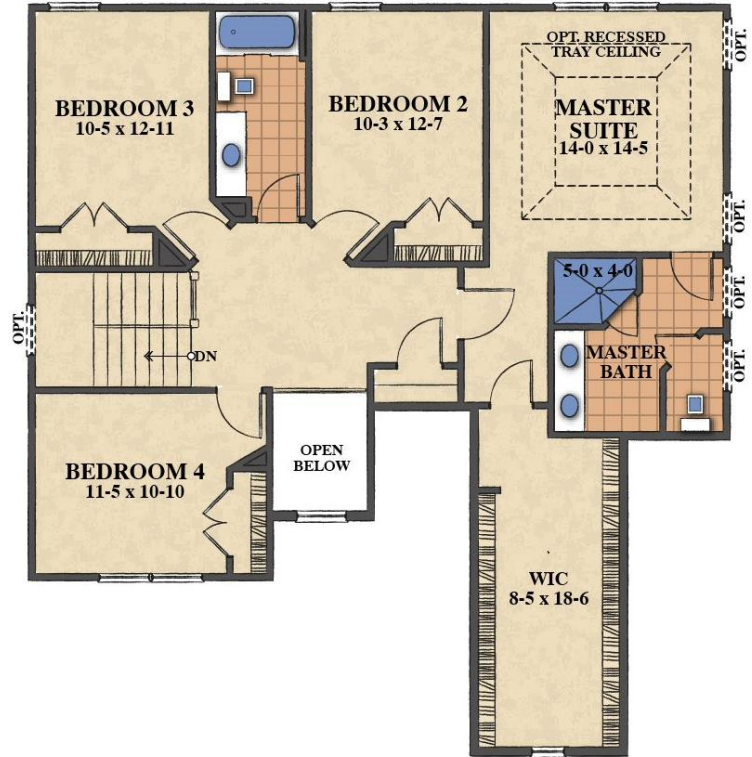
INCLUDED SECOND FLOOR LAYOUT
