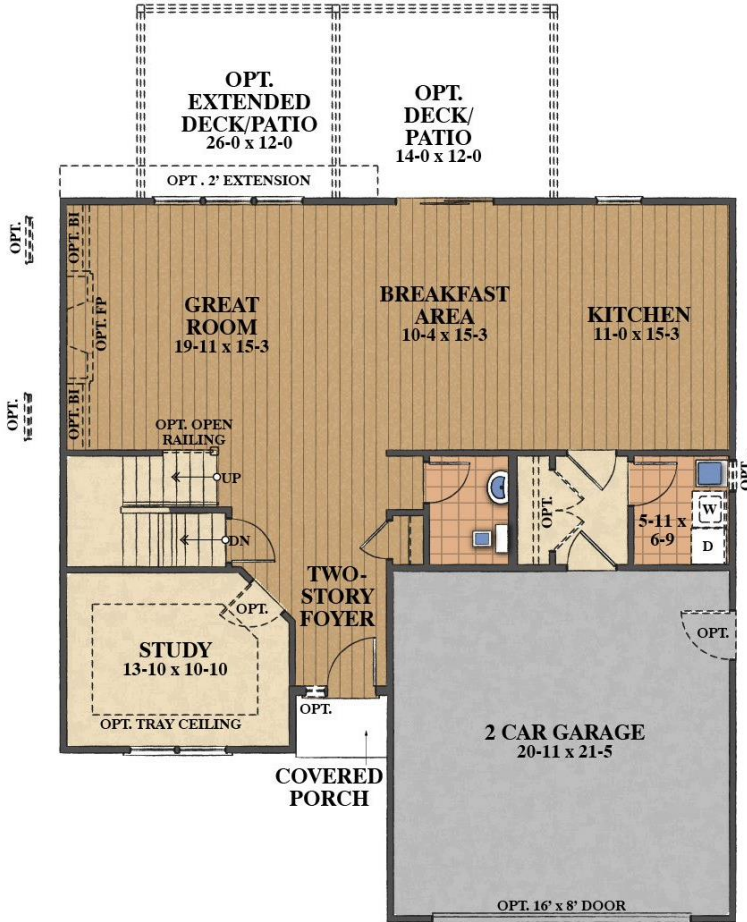
INCLUDED FIRST FLOOR LAYOUT
