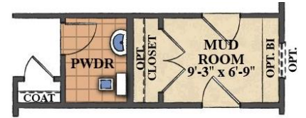
OPT. MUD ROOM LAYOUT W/ OPT. SECOND FLOOR LAUNDRY
