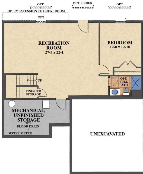
OPTIONAL FINISHED BASEMENT LAYOUT
